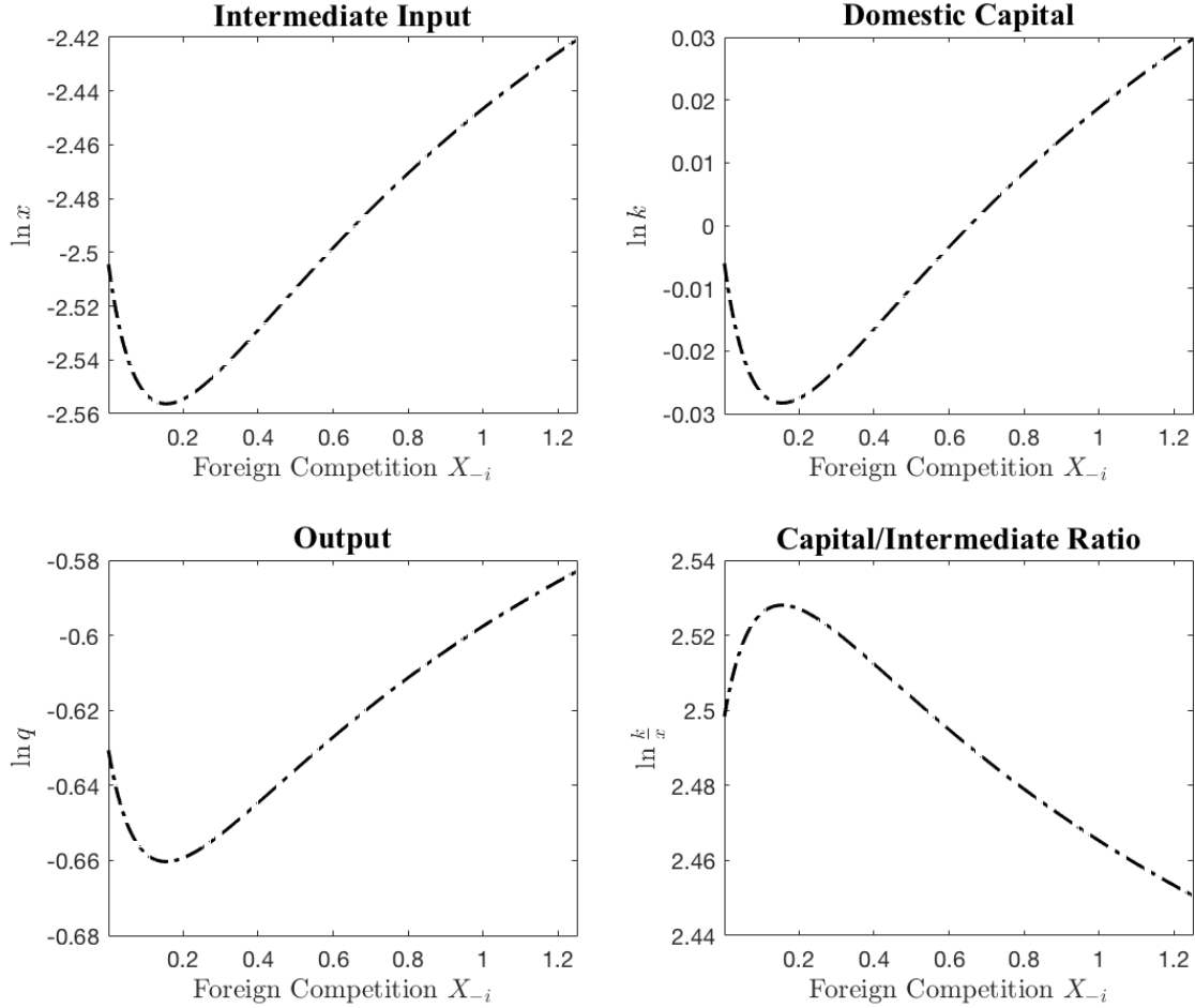
Figure 5: Firm-level Equilibrium as a Function of Foreign Competition X_{-i}
