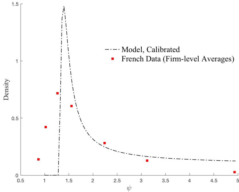
Figure 6: Buyer Power and Domestic Share of Input Expenditure, Model vs. Data
