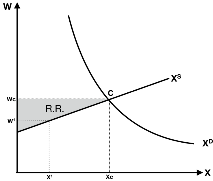
Figure A.2: Ricardian Rents
