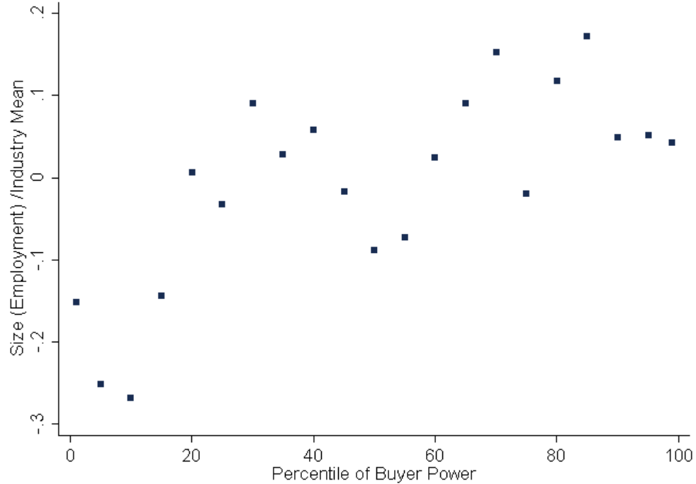
Figure A.1a: Input Market Power and Firm Size, Regime “BP”
