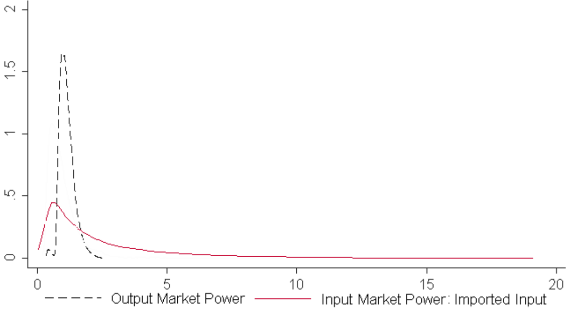
Figure A.4: Market Power in Input and Output Market, FULL SAMPLE
